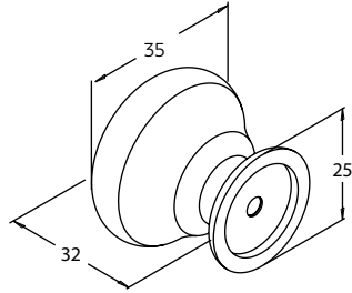
Knob Part no. TCM3620
