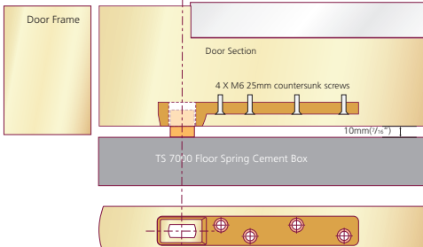
Bottom Door Fitting (Bottom View)
